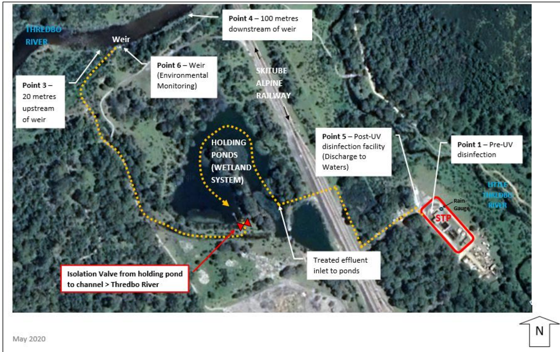
Figure 9.1 Site Map showing monitoring points and flow path from STP > holding ponds > channel > Thredbo River
